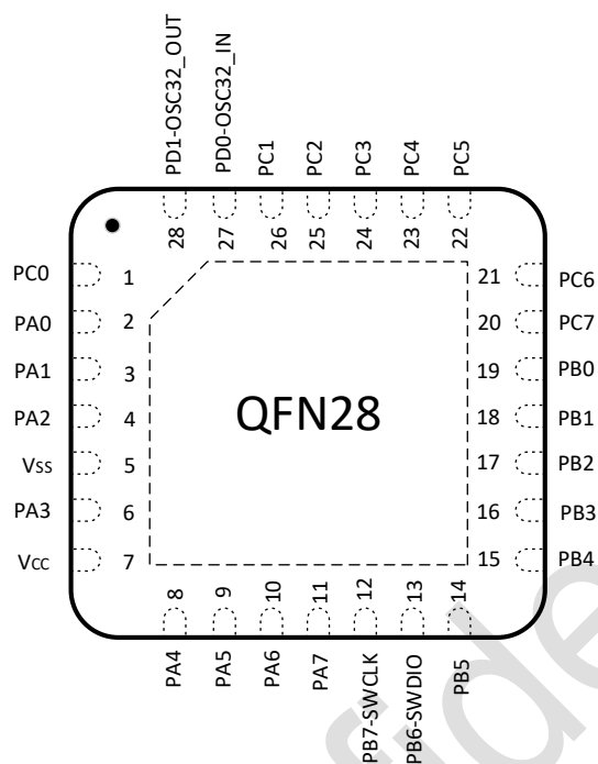
图 3-1 QFN28 Pinout1 PY32CA80G1xU7 (Top view)
