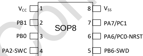
图 3-6 SOP8 Pinout1 PY32F002BL15Sx (Top view)
